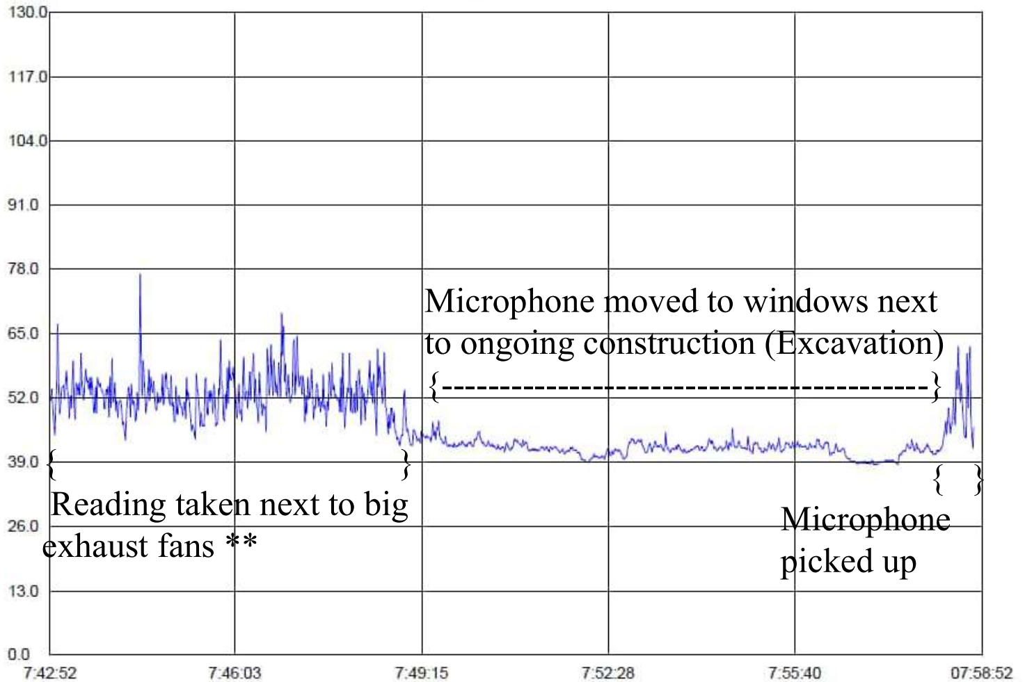
Standard Sound Level Meter RealTime Graph Time: 2019-9-3 13:56:51
