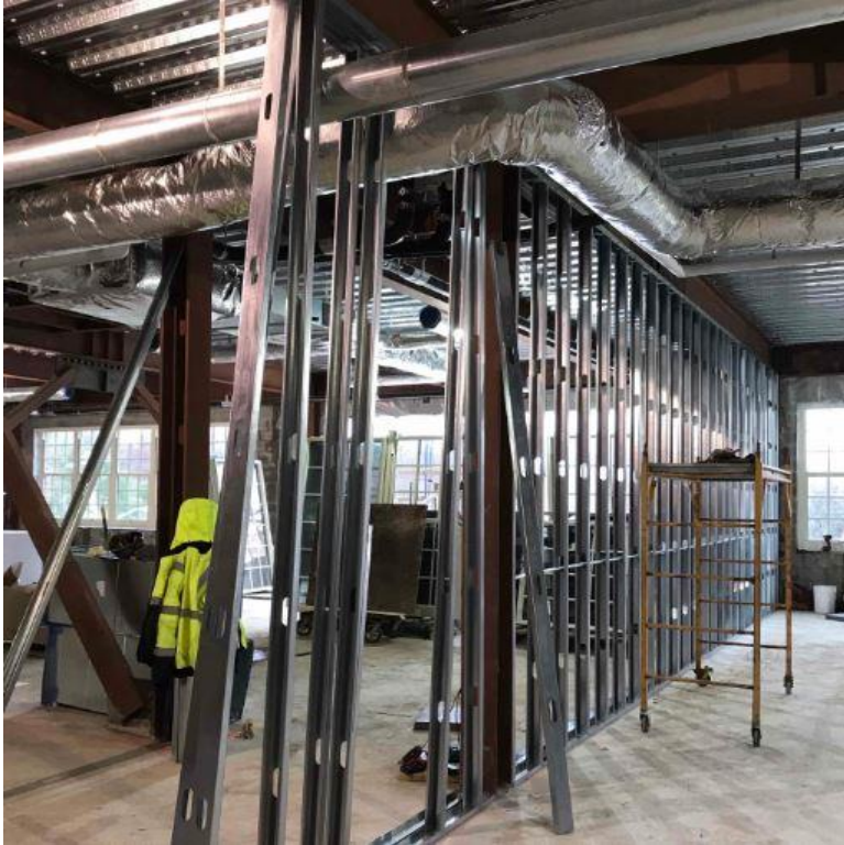
Light Gauge Metal Framing at 2 nd Floor of New Addition
