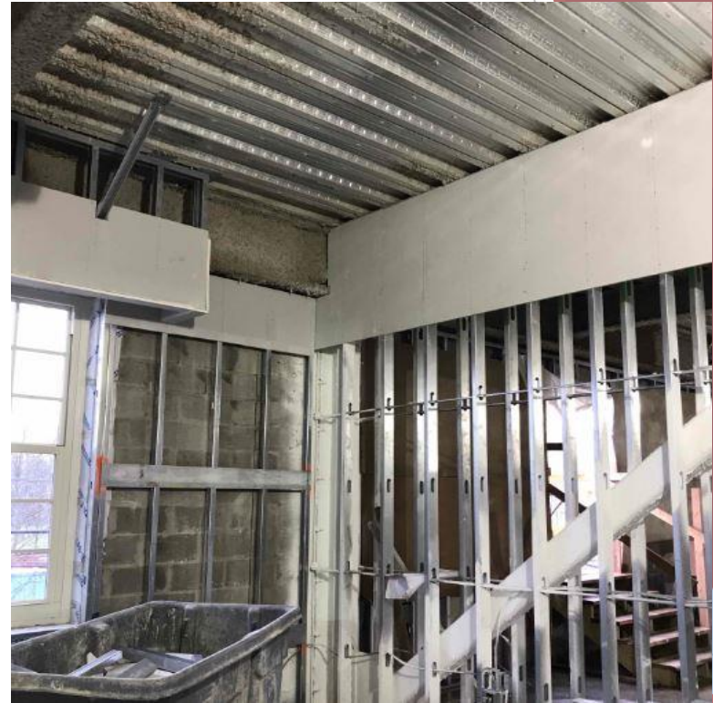
Installation of Sheetrock Wall Finishes at 1 st Floor of New Addition
