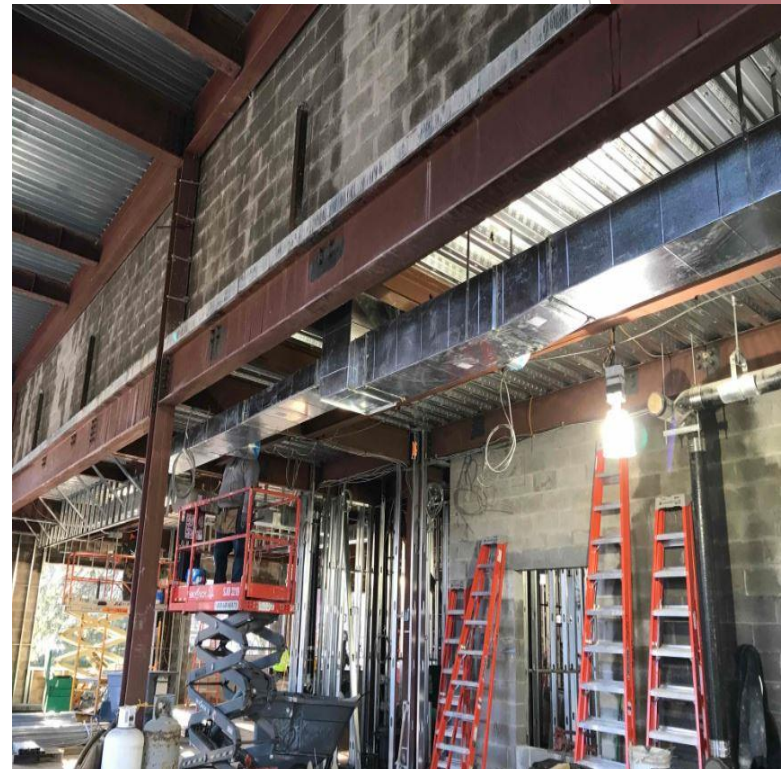
Installation of HVAC duct work at Learning Commons 146
