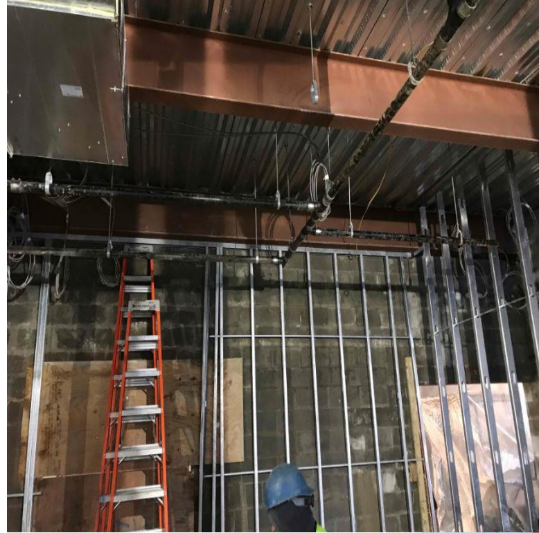
Installation of overhead plumbing piping at Kitchen
