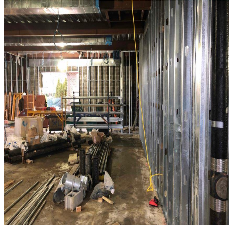
Construction of light gauge metal frame interior partitions at MPR Room 145
