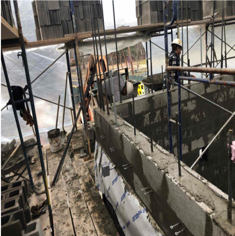
Construction of stairwell 163 CMU partitions
