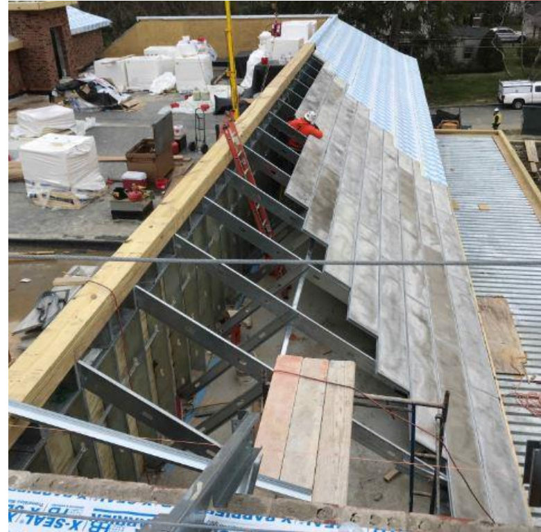
Installation of concrete roof planking
