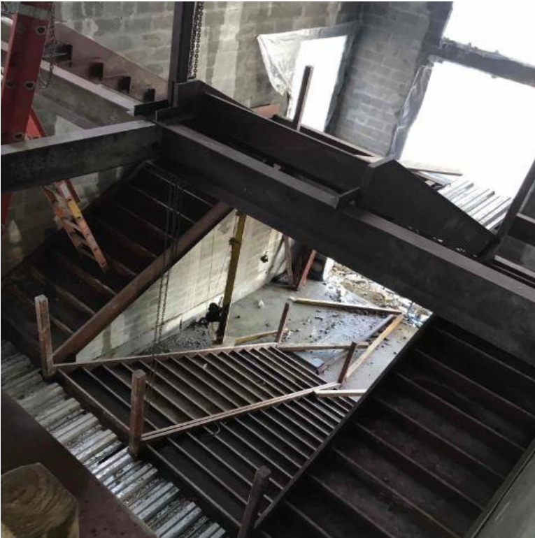
Installation of staircase 163
